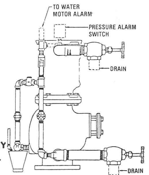
SPRINKLER SYSTEM
