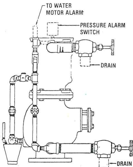
SPRINKLER SYSTEM
